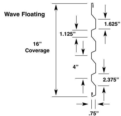
Wave Floating
