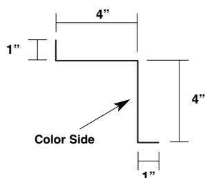
Inside Corner Trim - Notched MT-WAV-CRN-IS-STD
