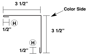
Outside Corner Trim MT-55
