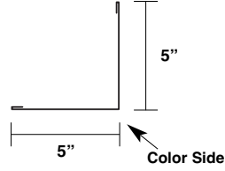
**Outside Corner Trim MT-197
