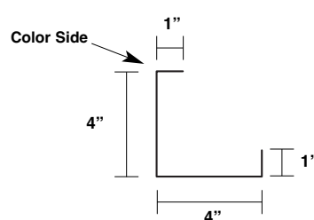
Outside Corner Trim - Notched MT-WAV-CRN-OS-STD
