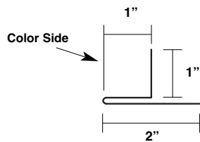
Outside Corner Cleat - Notched (Left) (Houston Plant Only) MT-174
