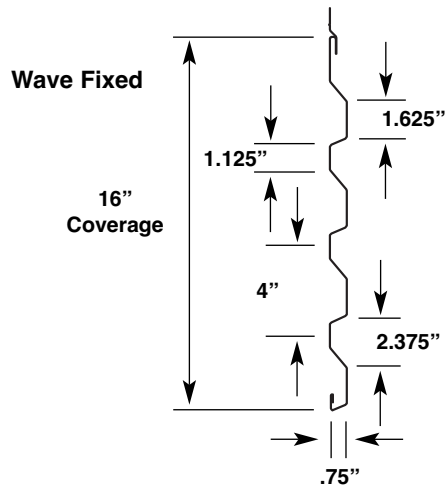
Wave Fixed
