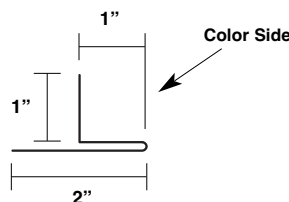
Outside Corner Cleat - Notched (Right) (Houston Plant Only) MT-175
