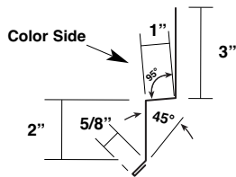
**Vertical Splice Trim MT-199
