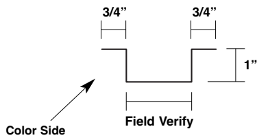
Reveal Closure MT-195
