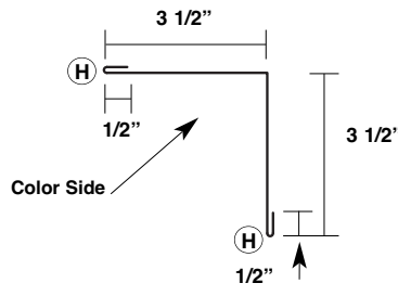
Inside Corner Trim MT-56
