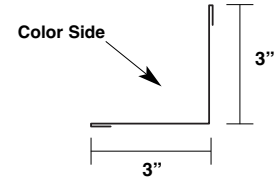
**Inside Corner Trim MT-198
