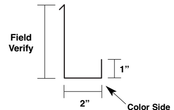
Jamb Trim - Notched (Right) (Houston Plant Only) MT-173R
