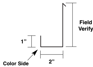
Jamb Trim - Notched (Left) (Houston Plant Only) MT-173L
