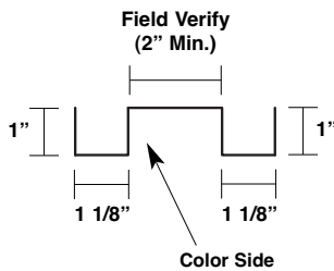
Vertical Reveal - Notched (Houston Plant Only) MT-172
