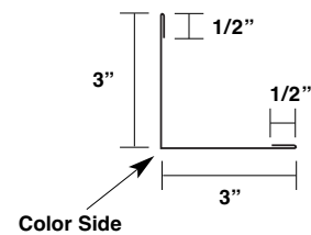
Outside Angle For Outside Corner 3" x 3"
