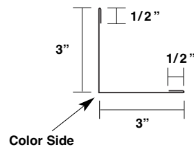
Outside Angle For Outside Corner 3" x 3"
