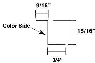
Zee Spacer MQZS
