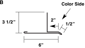
Soffit Base Trim MQSB
