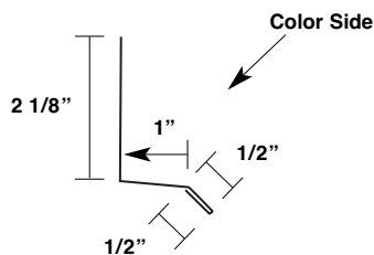
Base & Drip Trim
