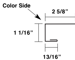
Panel Cap Trim MQPC
