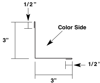
Inside Angle for Inside Corner 3" x 3"
