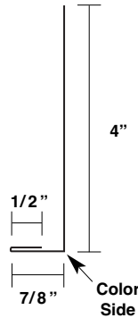
Angle Trim 7/8" x 4"
