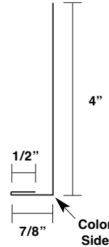
Angle Trim 7/8" x 4"
