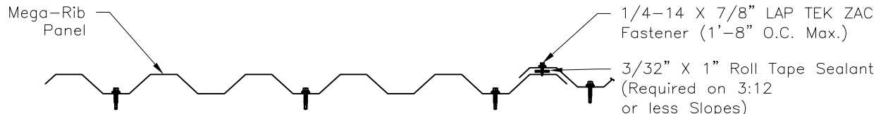
FASTENER PATTERN (@ Intermediate Purlins)
