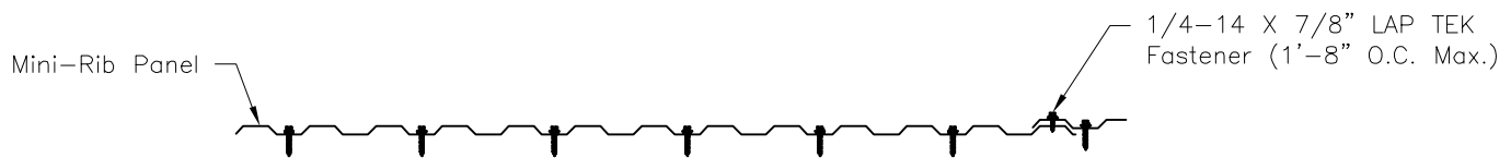
FASTENER PATTERN (@ Eaves, Ridges & Endlaps)
