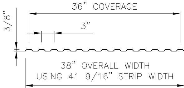
MINI-RIB PROFILE
