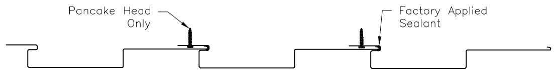
CUSTOM REVEAL SEAM ENGAGEMENT
