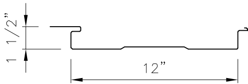
INVERTED PLANK PROFILE
