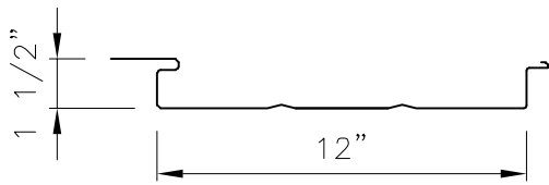
VEE GROOVES PROFILE
