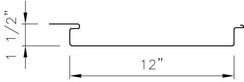
FLAT PROFILE
