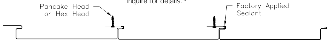
TYPICAL SEAM ENGAGEMENT
